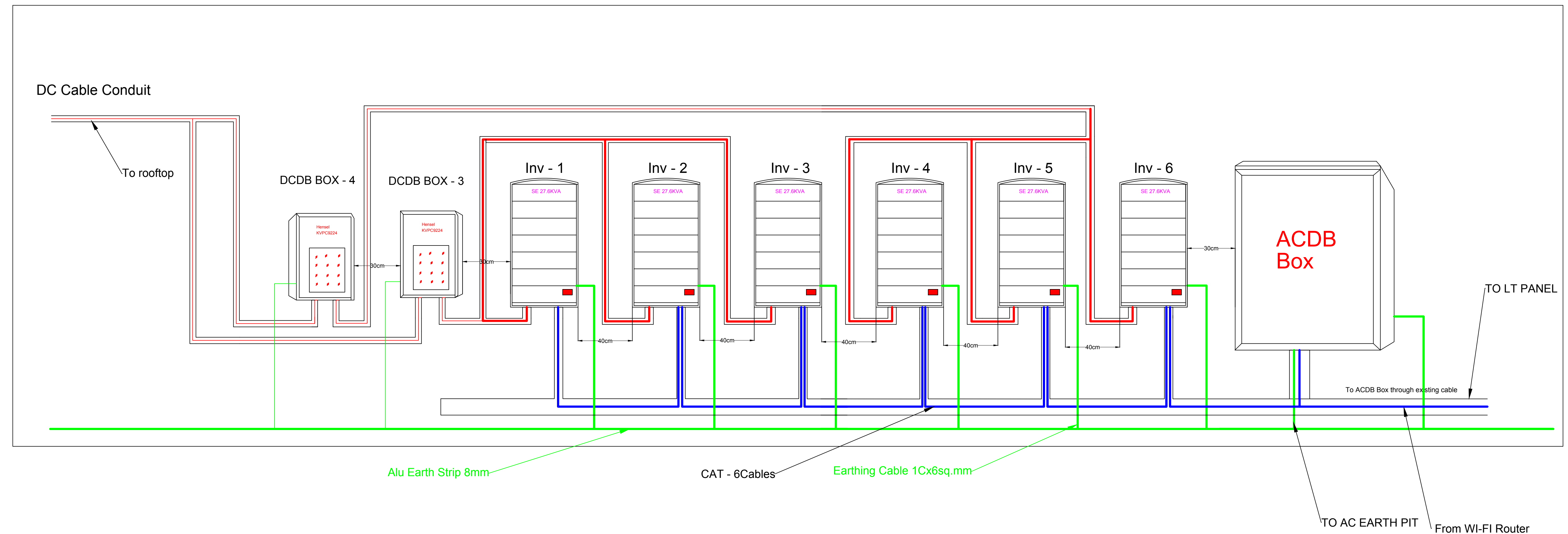
Interconnection point
