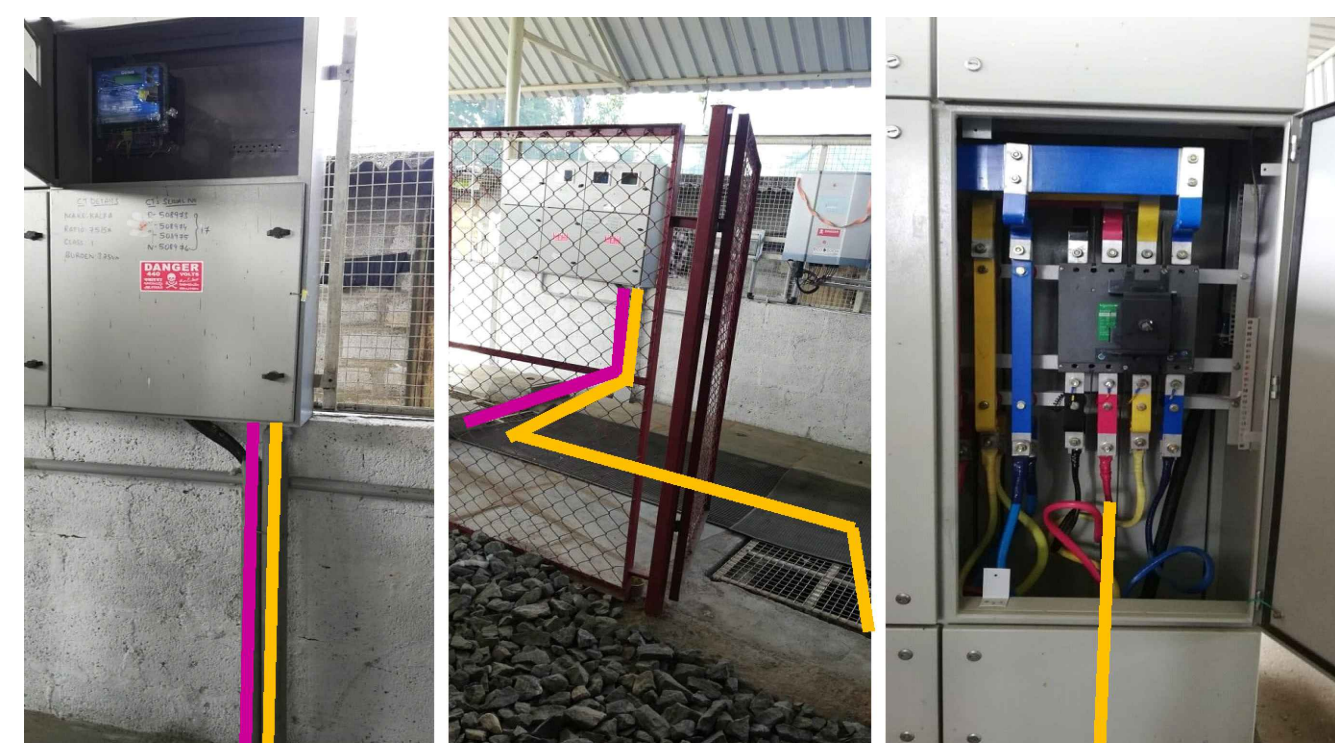
AC CABLE ROUTING FROM METER CUBICAL TO LT PANEL
